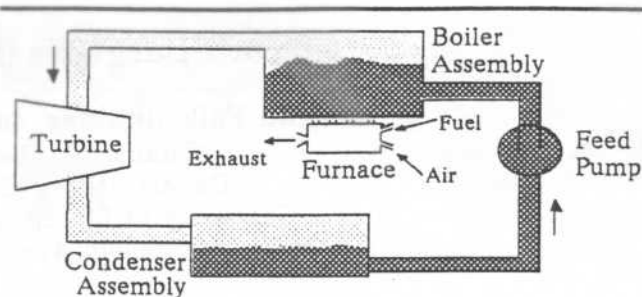
Figure 1: Simplified model of a navy steam-powered propulsion plant.
