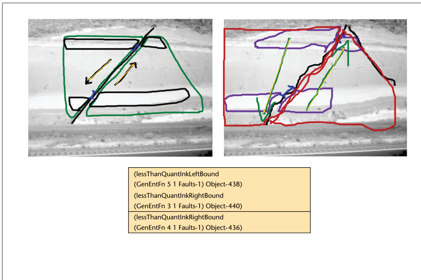
Figure 2. Two Sketches That Are Frequently Clustered Together and Three High-Probability Facts from Their Generalization.
