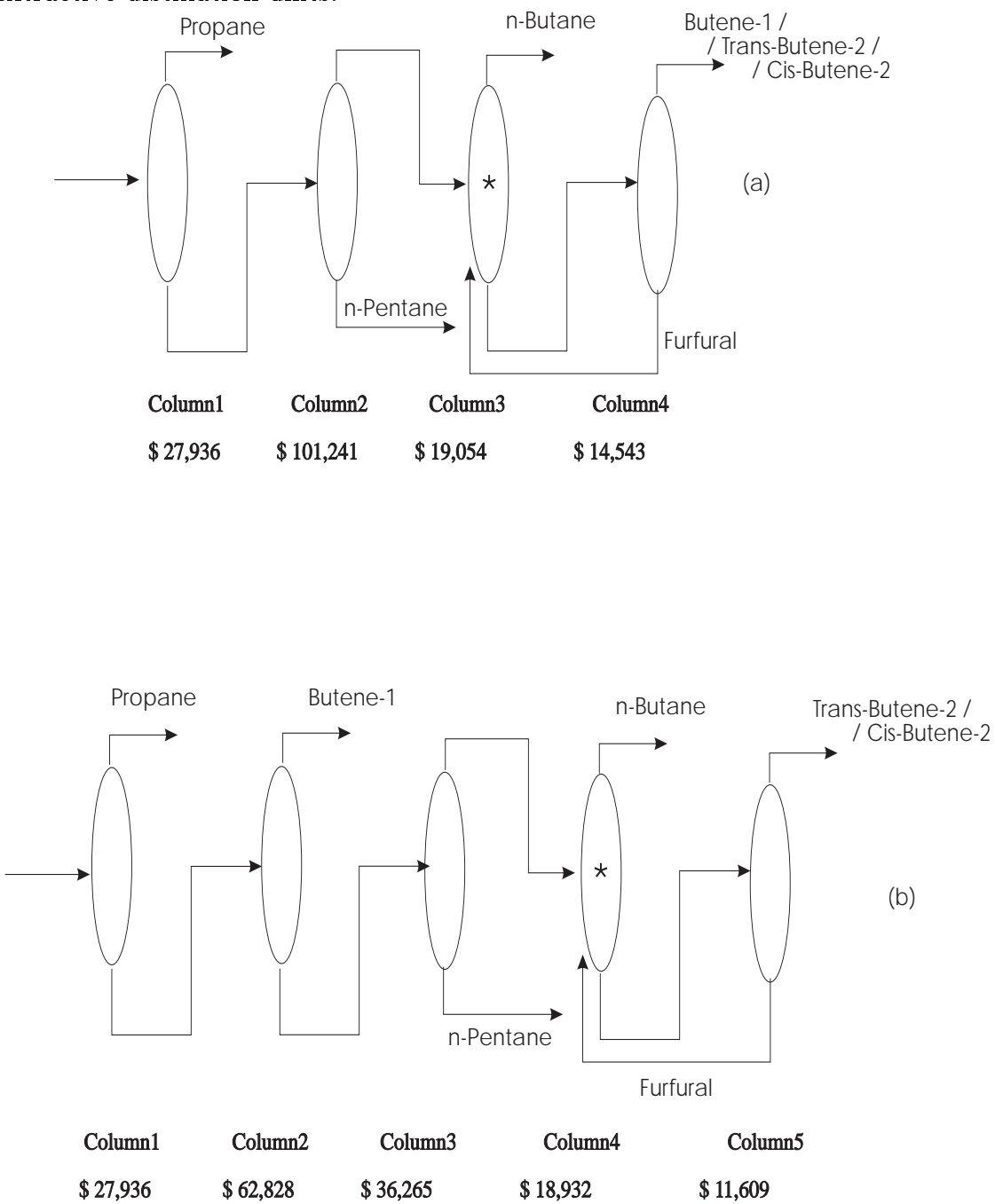
Figure 6.11: The first two flowsheets generated by the Nath & Notard method for the n-Butylene purification problem. The columns with an asterisk (*) indicate extractive distillation units.
