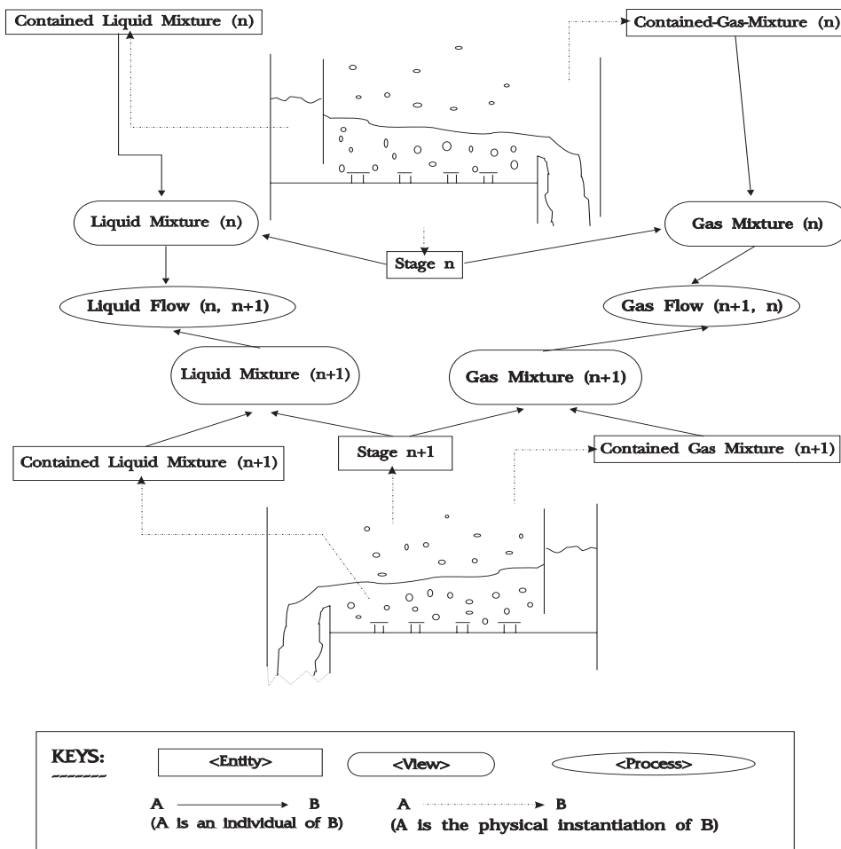
Figure 4.11: Model fragments that describe the physical activity between two successive stages in a column.
