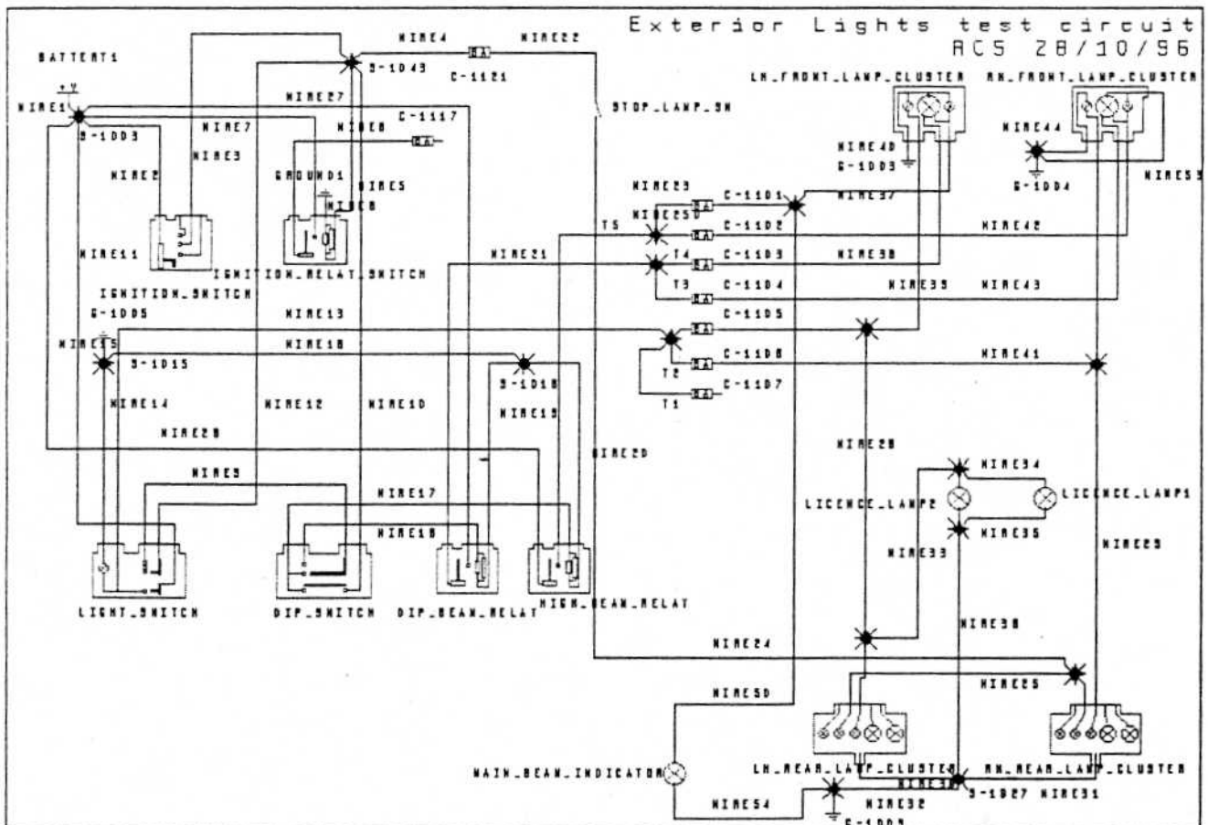
Figure 1 : Traditional lighting circuit
