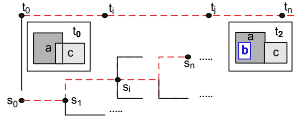
Figure 4: Branching-time Situation History
