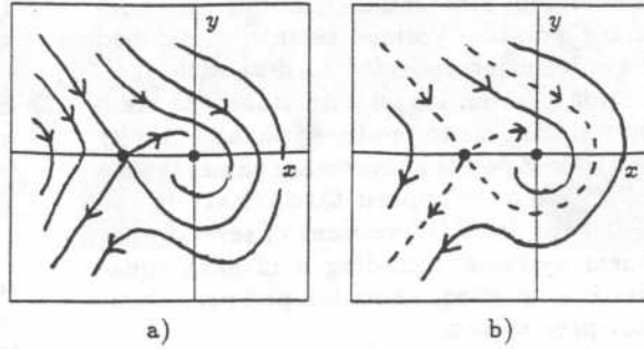
Figure 1: Phase portraits of the Lienard equation: a) from [Brauer & Nohel 69] and [Sacks 90], and b) from QPORTRAIT.
