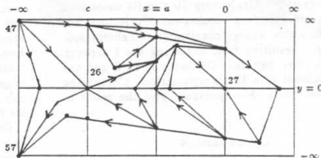
a) Envisionment graph of the Lienard equation in the phase plane.
