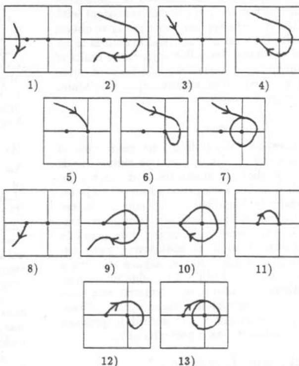
b) Trajectories from initial gathering. Trajectories 7 and 13 are cyclic and incomplete. Trajectory 10 is a homoclinic orbit.
