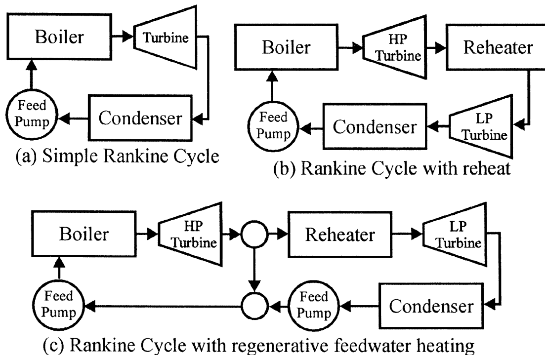
Figure 1: Sequence of conceptual designs for a power plant
